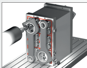
Complex pieces on magnetic cube or tombstone
