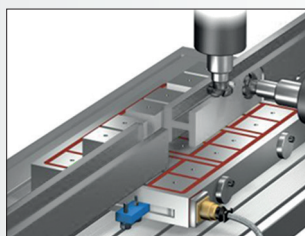
Machining of profiles with magnetic stop on horizontal / vertical spindle machine
