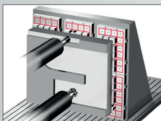
Face milling, edge milling, drilling on horizontal spindle machine
