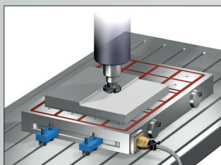
Face milling on vertical spindle machine
