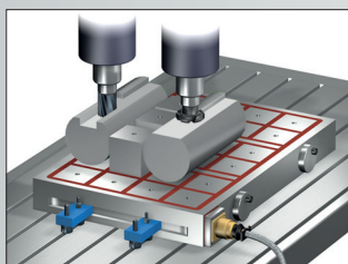
Machining of steel rounds with side mechanical / magnetic stop
